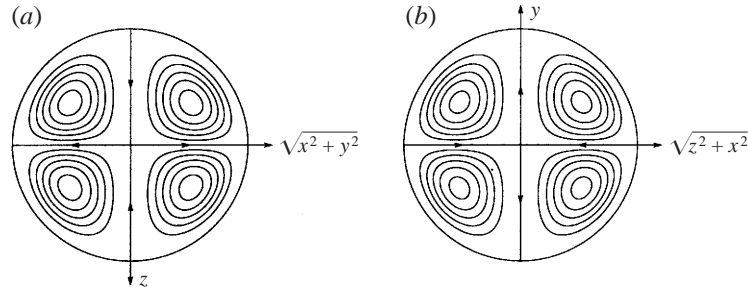
FIGURE 3. Streamlines in meridian planes of the first-order flow corrections due to (a) inertia, \mathbf{u}_{1I} , and (b) buoyancy \mathbf{u}_{1B} .
