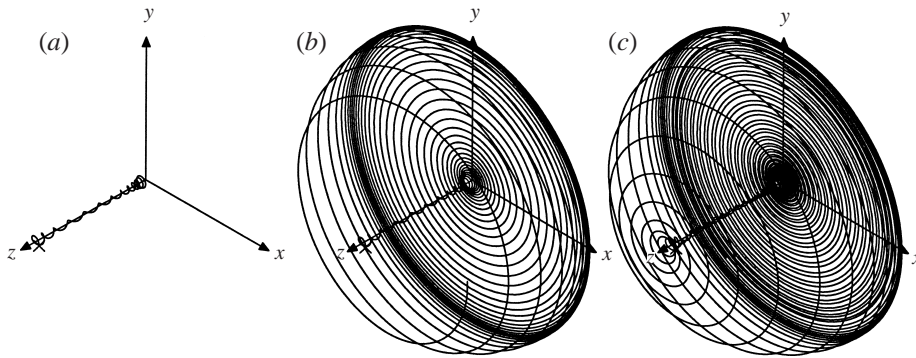
FIGURE 4. The trace of a particle released at the point r = 0.45 , \theta = \phi = 0.05 , marked \times , into the flow \mathbf{u}_0 + Gr \mathbf{u}_1 with Ra = 1000 , Pr = 0.7 after a dimensionless time interval (units of D^2/\nu Gr ) of (a) 10 000, (b) 240 000, and (c) 360 000.
